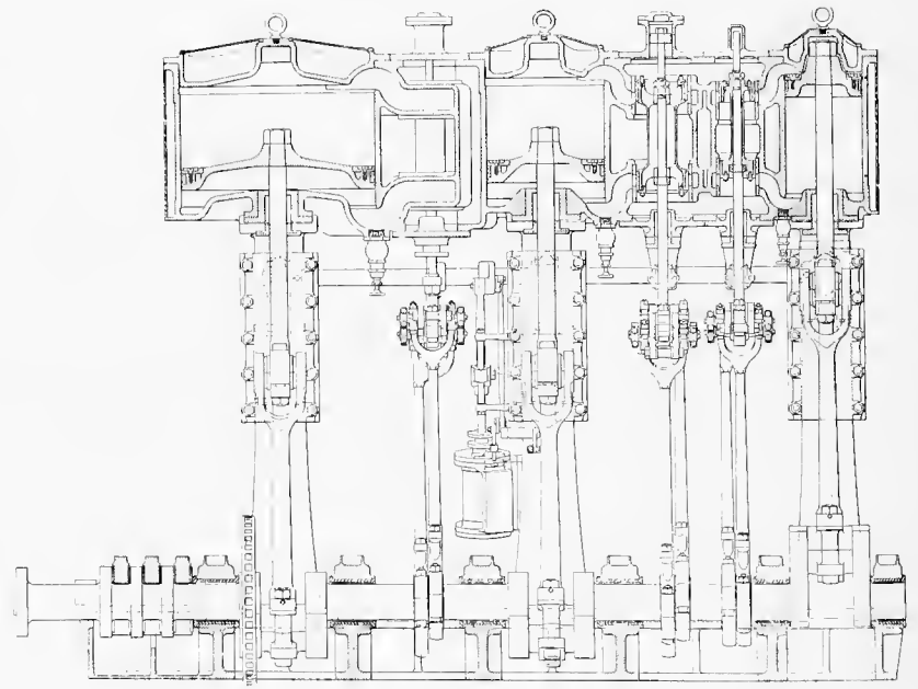
TRIPLE-EXPANSION ENGINE OF H. W. SIBLEY'S STEAM YACHT RESTLESS.—Built by F. W. Wheeler & Co., West Bay City, Mich.
